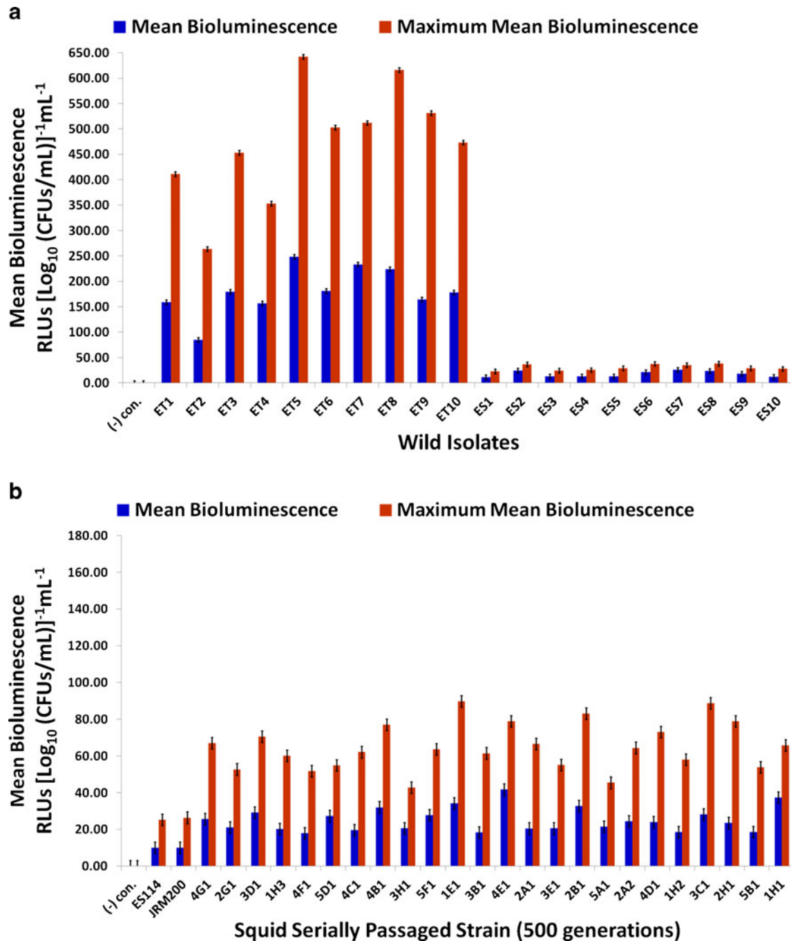
Fig. 7 Mean and maximum mean bioluminescence for a wild V. fischeri strains from E. tasmanica (“ET”) and E. scolopes (“ES”) specimens collected from the field and b ancestor V. fischeri ES114, unevolved JRM200, and the 24 lines evolved through the novel Australian squid host E. tasmanica for 500 generations ( n=6 ). Error bars represent Fisher
