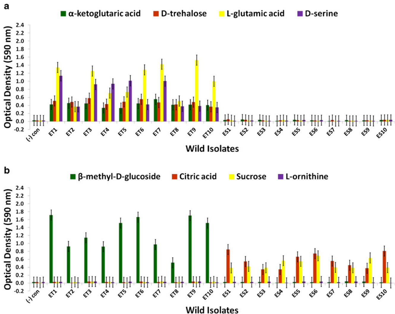
Fig. 4 Optical density (590 nm) measurements in a \alpha -ketoglutaric acid, D-trehalose, L-glutamic acid, and D-serine, and b \beta -methyl-D-glucoside, citric acid, sucrose, and L-ornithine of wild V. fischeri isolates from Australian E. tasmanica (“ET”) and Hawaiian E. scolopes (“ES”) specimens collected from the field ( n=3 ). Error bars represent Fisher LSDs
