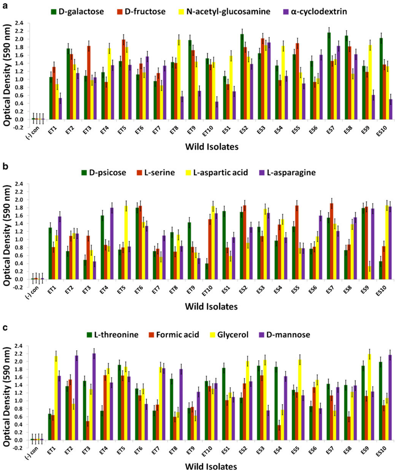
Fig. 3 Optical density (590 nm) measurements in a D-galactose, D-fructose, N-acetyl-D-glucosamine, and \alpha -cyclodextrin; b D-psicose, L-serine, L-aspartic acid, and L-asparagine; and c L-threonine, formic acid, glycerol, and D-mannose of wild V. fischeri isolates from E. tasmanica (“ET”) and E. scolopes (“ES”) specimens collected from the field ( n=3 ).
